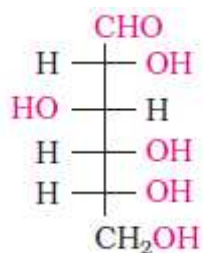
D- Glucose (Open chain structure)
